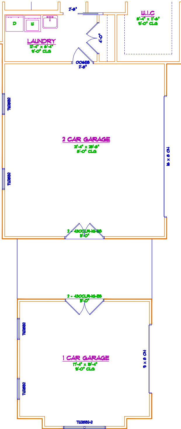
3 CAR GARAGE OPTION
